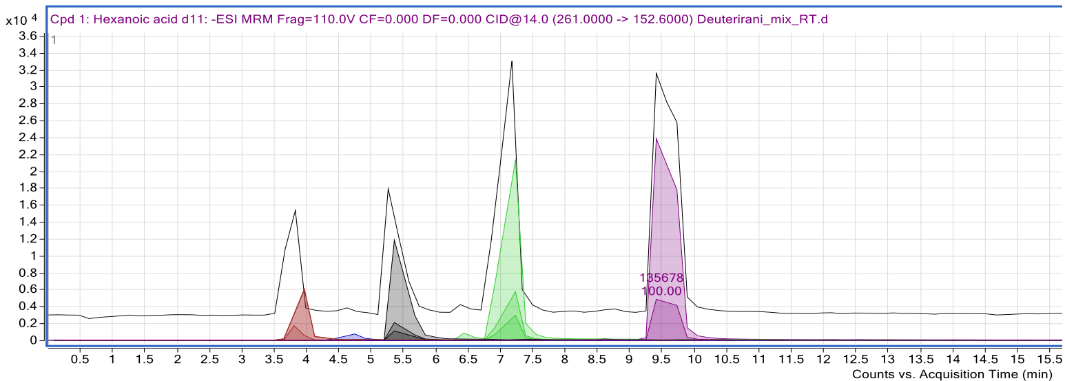
Figure 7. MS spectrum showing acetic acid d 4 (red), propionic acid d 3 (blue), butyric acid d 7 (grey), pentanoic acid d 9 (green), hexanoic acid d 11 (purple), in order by their retention time (R T ).
