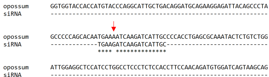
Figure 15 A single nucleotide mismatch between commercially available ACTB siRNA and siRNA-binding site on the predicted opossum ACTB gene sequence. Aligned nucleotides are marked with asterisks. There is one mismatch (arrow) at the position 5 of the ACTB siRNA.
