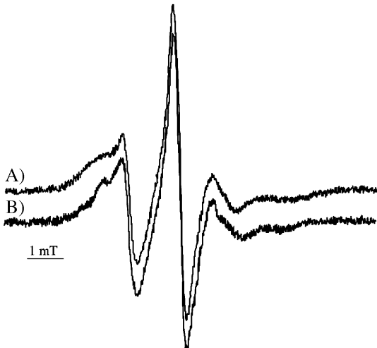
Fig. 4. Experimental spectra of control and cadmium-treated brush border membrane at 32 °C.
