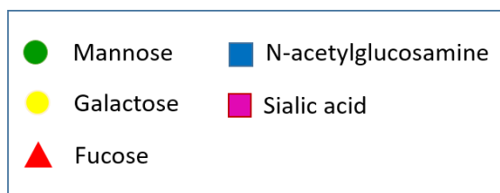
Figure 26. Glycan legend
