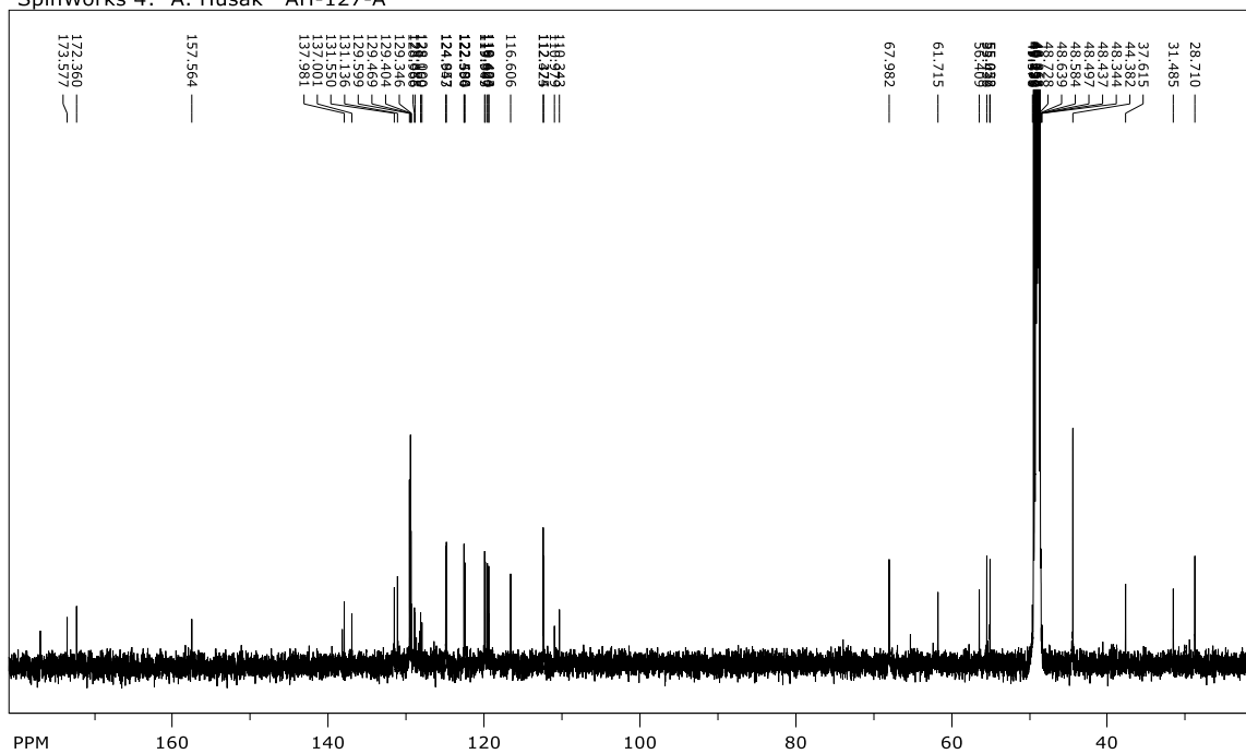
Prilog 57. ^{13}\text{C} NMR ( \text{CD}_3\text{OD} , 150 MHz) spektr 2\text{HCl}\times\text{H-Trp-Trp-Tyr}[\text{CH}_2\text{N}(\text{CH}_3)_2]\text{-OBn} (36)
