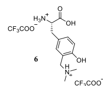
Prilog 10. ^1\text{H} NMR ( \text{CD}_3\text{OD} , 300 MHz) spektar 2\text{TFA}\times\text{H-Tyr}[\text{CH}_2\text{N}(\text{CH}_3)_2]\text{-OH} (6)
