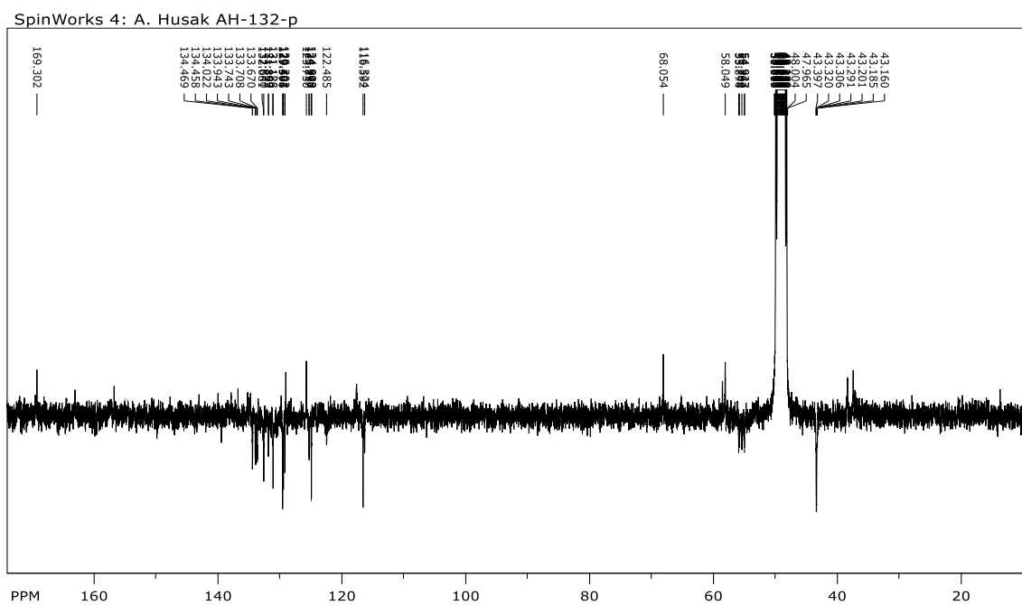
Prilog 66. ^{13}\text{C} NMR ( \text{CDCl}_3 , 75 MHz) spekter 3\text{HCl}\times\text{H-Phen-Tyr}[\text{CH}_2\text{N}(\text{CH}_3)_2]\text{-OBn} ( 41 )
