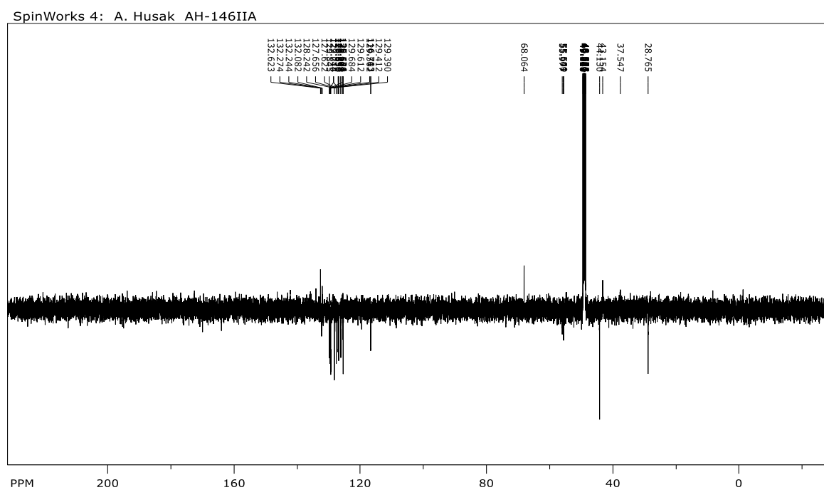
Prilog 68. ^{13}\text{C} NMR ( \text{CD}_3\text{OD} , 75 MHz, APT) spektar Boc-Pyr-Tyr[ \text{CH}_2\text{N}(\text{CH}_3)_2 ]-OBn ( 42 )
