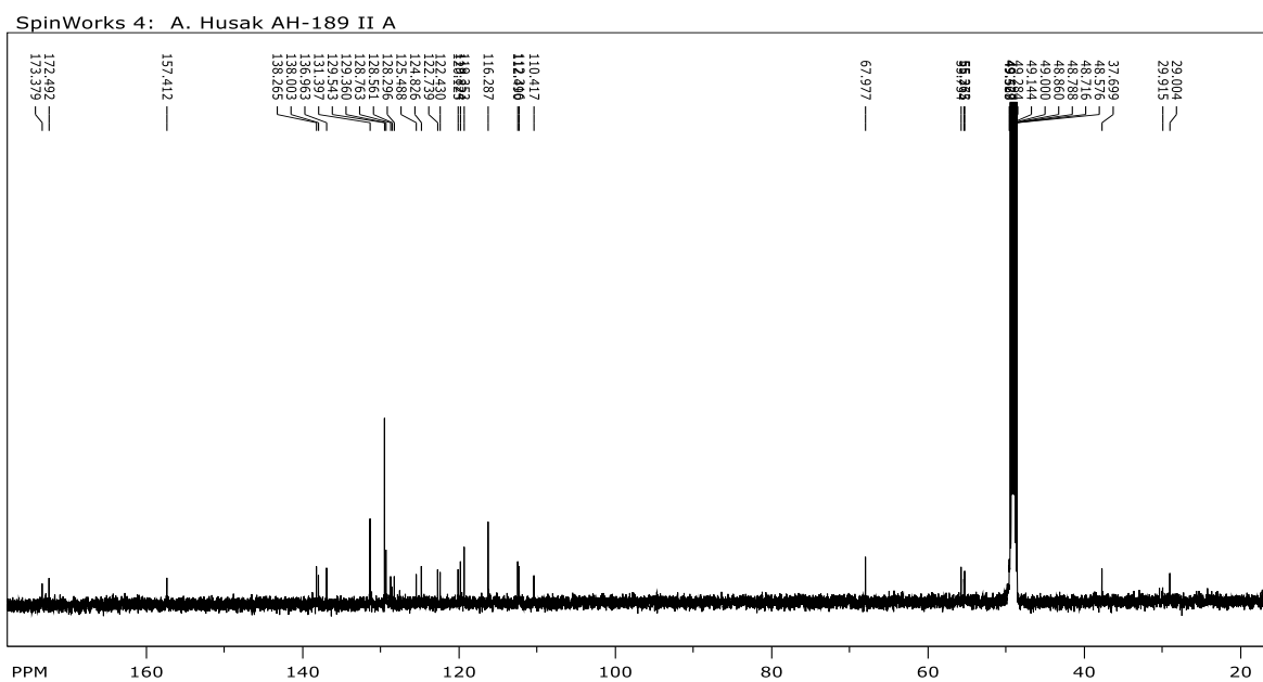
Prilog 55. ^{13}\text{C} NMR ( \text{CD}_3\text{OD} , 150 MHz) spektar \text{HCl} \times \text{H-Trp-Trp-Tyr-OBn} ( 35 )
