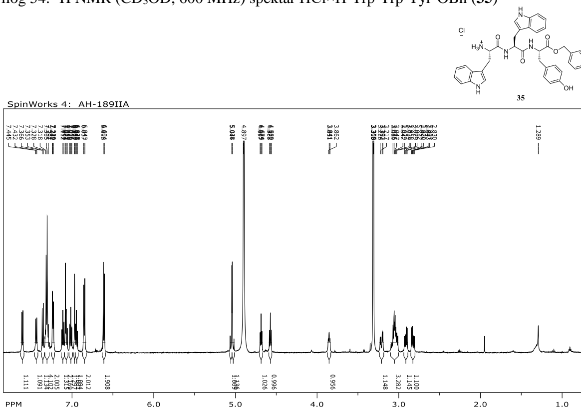
Prilog 54. ^1\text{H} NMR ( \text{CD}_3\text{OD} , 600 MHz) spektar \text{HCl} \times \text{H-Trp-Trp-Tyr-OBn} ( 35 )
