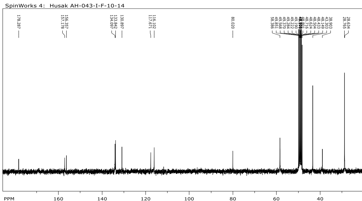
Prilog 7. 13 C NMR (CD 3 OD, 75 MHz) spektar Boc-Tyr[CH 2 N(CH 3 ) 2 ]-OH ( 4 )
