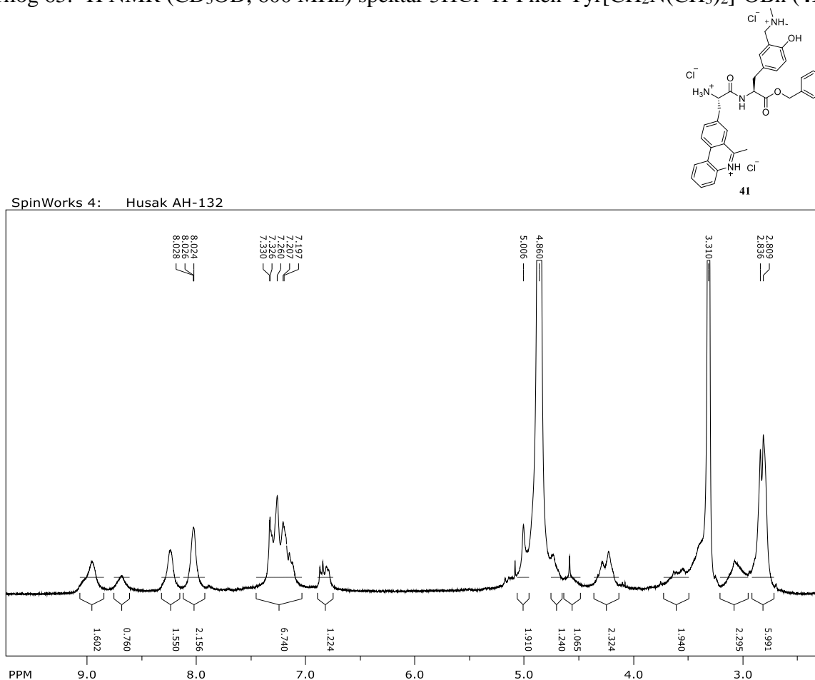
Prilog 65. ^1\text{H} NMR ( \text{CD}_3\text{OD} , 600 MHz) spekter 3\text{HCl}\times\text{H-Phen-Tyr}[\text{CH}_2\text{N}(\text{CH}_3)_2]\text{-OBn} ( 41 )
