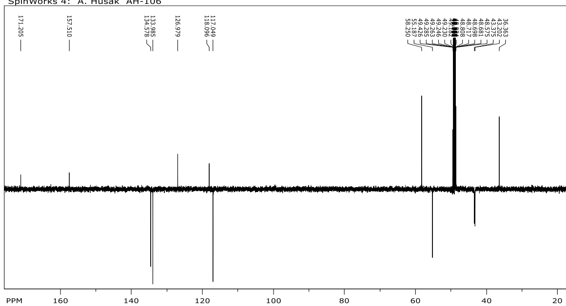
Prilog 11. ^{13}\text{C} NMR ( \text{CD}_3\text{OD} , 75 MHz) spektar 2\text{TFA}\times\text{H-Tyr}[\text{CH}_2\text{N}(\text{CH}_3)_2]\text{-OH} (6)
