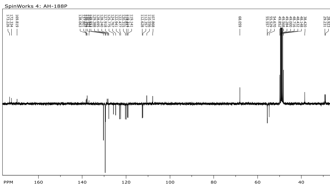
Prilog 53. ^{13}\text{C} NMR ( \text{CD}_3\text{OD} , 75 MHz) spektar \text{HCl}\times\text{H-Trp-Trp-Phe-OBn} ( 34 )
