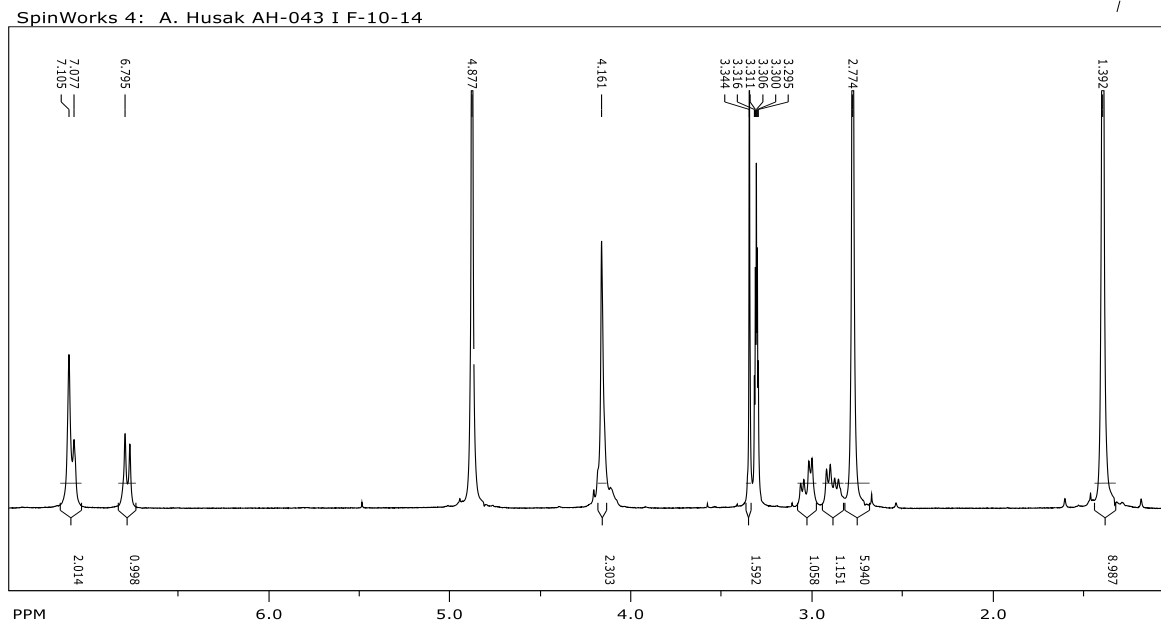
Prilog 7. 13 C NMR (CD 3 OD, 75 MHz) spektar Boc-Tyr[CH 2 N(CH 3 ) 2 ]-OH ( 4 )
