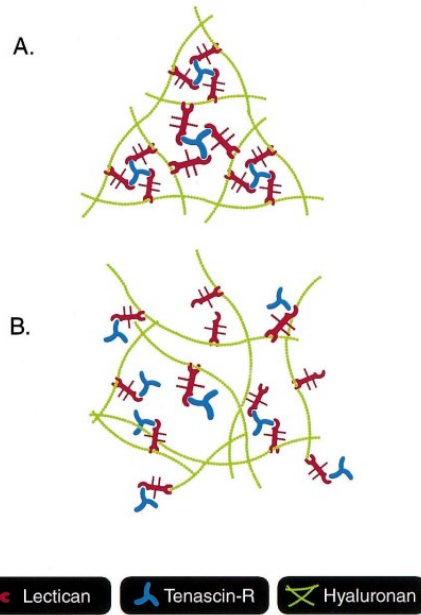
Figure 5 Quaternary complexes form PNNs (link proteins not shown) [30]
