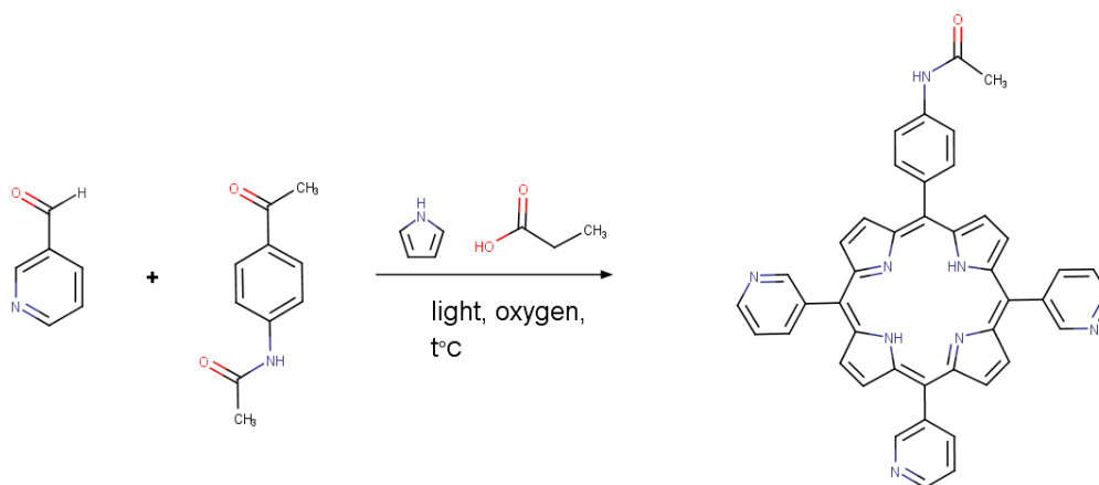
Figure 7: Synthesis of porphyrin 2
