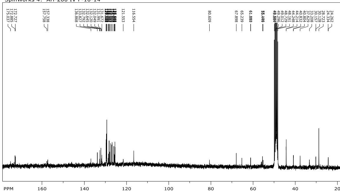
Prilog 79. ^{13}\text{C} NMR ( \text{CD}_3\text{OD} , 75 MHz) spektar Boc-Lys(Pyr)-Tyr[ \text{CH}_2\text{N}(\text{CH}_3)_2 ]-OBn (49)
