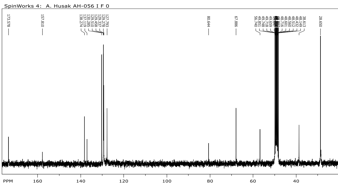
Prilog 16. 13 C NMR (CD 3 OD, 75 MHz) spektar Boc-Phe-OBn (9)
