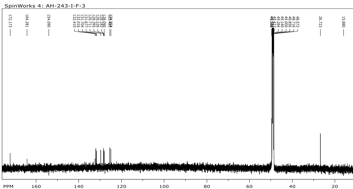
Prilog 70. 13 C NMR (CD 3 OD, 150 MHz) spektar Pyr-OSu ( 43 )
