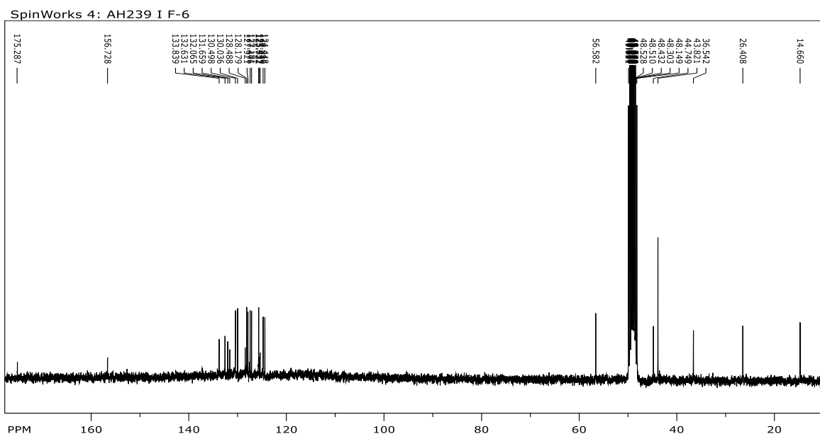
Prilog 72. 13 C NMR (CD 3 OD, 75 MHz) spektar Pyr-EDC ( 44 )
