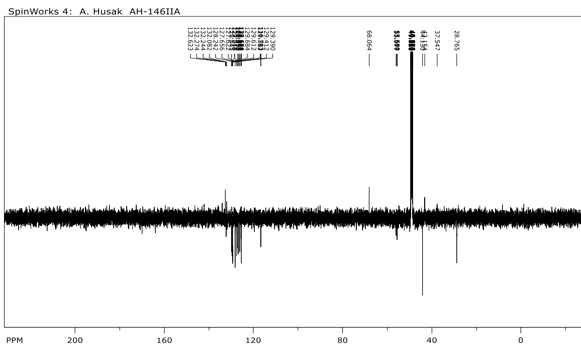
Prilog 68. 13 C NMR (CD 3 OD, 75 MHz, APT) spektr Boc-Pyr-Tyr[CH 2 N(CH 3 ) 2 ]-OBn (42)
