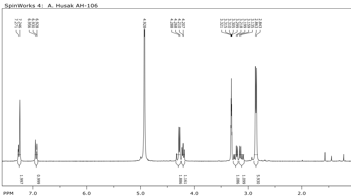
Prilog 11. ^{13}\text{C} NMR ( \text{CD}_3\text{OD} , 75 MHz) spektar 2\text{TFA}\times\text{H-Tyr}[\text{CH}_2\text{N}(\text{CH}_3)_2]\text{-OH} (6)
