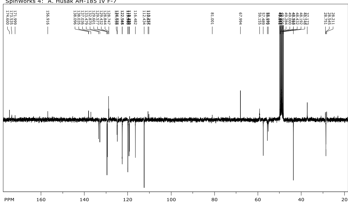
Prilog 51. ^{13}\text{C} NMR ( \text{CD}_3\text{OD} , 75 MHz) spektr Boc-Trp-Trp-Tyr[ \text{CH}_2\text{N}(\text{CH}_3)_2 ]-OBn (33)
