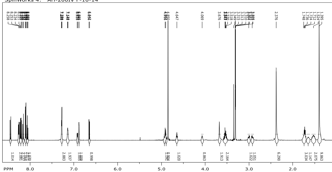
Prilog 79. ^{13}\text{C} NMR ( \text{CD}_3\text{OD} , 75 MHz) spektar Boc-Lys(Pyr)-Tyr[ \text{CH}_2\text{N}(\text{CH}_3)_2 ]-OBn (49)
