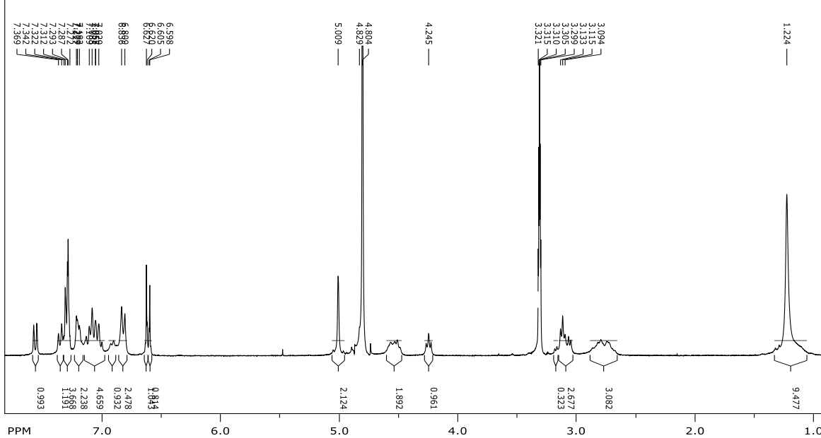
Prilog 49. ^{13}\text{C} NMR ( \text{CD}_3\text{OD} , 75 MHz) spektar Boc-Trp-Trp-Tyr-OBn ( 32 )
