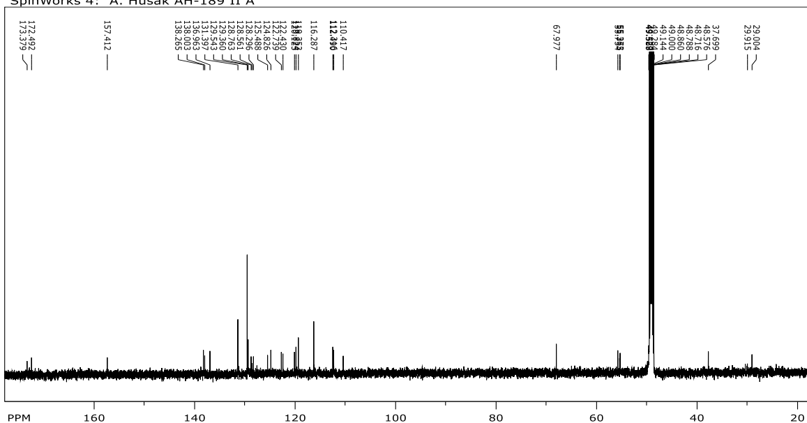
Prilog 55. 13 C NMR (CD 3 OD, 150 MHz) spektar HCl×H-Trp-Trp-Tyr-OBn ( 35 )
