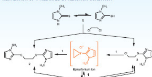
Scheme 1. Synthesis and interconversion of compounds 2, 3 and 4.
