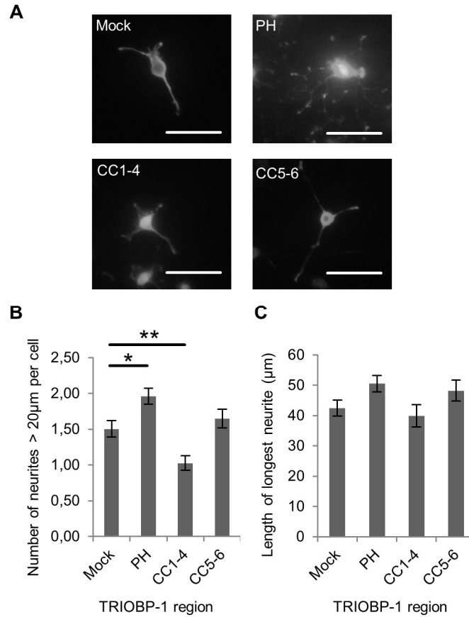
FIGURE 8: The effect of TRIOBP-1 subdomains on neurite outgrowth. (A) Sample images of Neurosreen-1 cells transfected with either an empty vector (“Mock”, n = 171) or one of the following TRIOBP-1 fragments: aa 60-189 (“PH”, n = 174), aa 281-555 (“CC1-4”, n = 161) and aa 556-652 (“CC5-6”, n = 152). Color has been deliberately over-exposed to ensure all neurites are visible. Scale bars represent 50 µm. (B) The mean number of neurites per cell (defined as any outgrowth over 20 µm in length) shows the PH domain alone to increase neurite number, and the central domain to decrease it. *: p < 0.05, **: p < 0.01 after correction for multiple testing. (C) Mean length of the longest neurite in each cell. The PH domain has a trend effect, significant before but not after correction for multiple testing. All values were compared by one-way ANOVA with Bonferroni correction to the “Mock” value.
