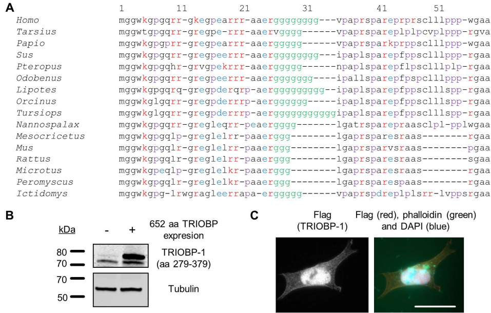
FIGURE 2; The extreme N-terminus of TRIOBP-1. (A) The putative initial 59 amino acids, aa, of TRIOBP-1, as present in multiple mammalian lineages. Notably, despite variation in amino acid sequence, and particularly in a poly-glycine stretch (green), all maintain the same reading frame. Positively charged residues are shown in red, negatively charged residues in blue and prolines in purple. Aligned using Clustal Omega (48) ( http://www.ebi.ac.uk/Tools/msa/clustalo ) and then manually curated. RefSeq accession number for the sequences shown are, in order displayed: NP_008963.3; XP_008065523.1; XP_009215517.1, XP_003126108.2; XP_006914811.1; XP_004410876.1; XP_007454108.1; XP_004279508.1; XP_004312195.1; XP_008849513.1; XP_005067025.1; XP_005067025.1; NP_001019887.1; XP_006242072.1; XP_005354277.1; XP_006979187.1; XP_005322324.1. (B) SH-SY5Y cells inducibly expressing the 652 aa species of TRIOBP-1, with and without induction of expression. The endogenous TRIOBP-1 species is seen to be of a slightly lower molecular weight than the 652 aa over-expressed protein, although a small amount of endogenous protein of this size is present, consistent with only a small portion of endogenous TRIOBP-1 protein expressing or maintaining the extreme N-terminus. (C) Expression of the N-terminal 59 aa of TRIOBP-1 alone in SH-SY5Y cells with a Flag tag.
